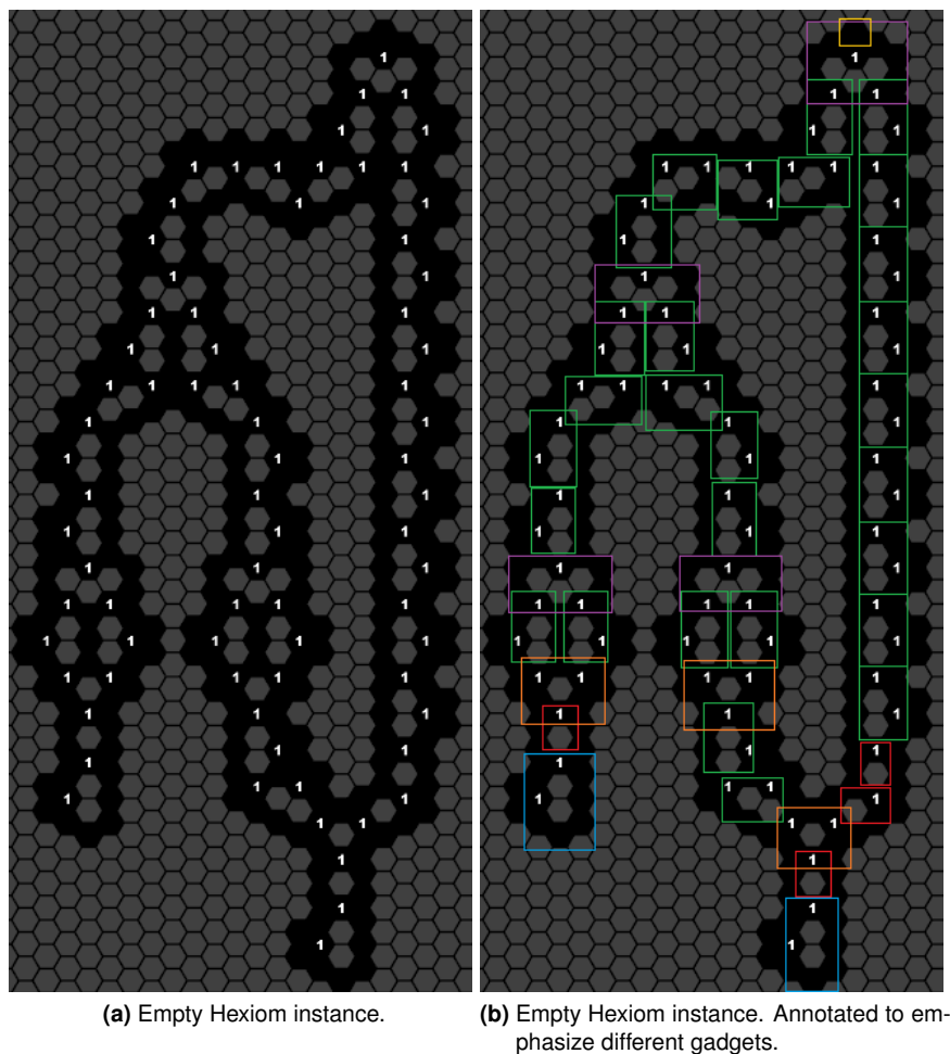
Figure A.11: Hexiom instance of the circuit (\neg x \wedge y) \vee x .
