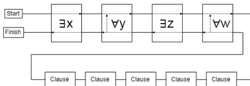
Figure 2.3: PSPACE-Hard framework from [1].
