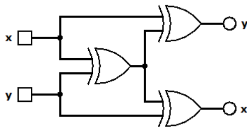
Figure 3.3: Crossover gadget using XOR gates.
