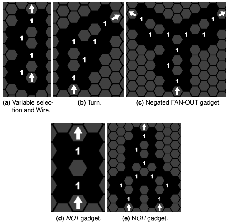
Figure 3.15: HexCells gadgets.
