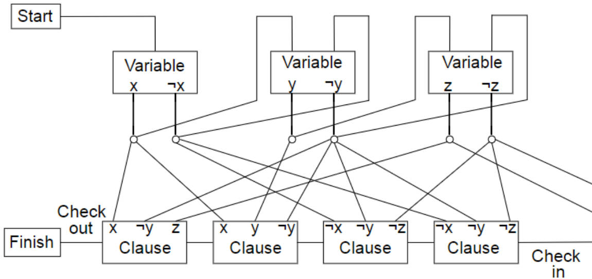
Figure 2.2: NP-Hardness framework from [1].
