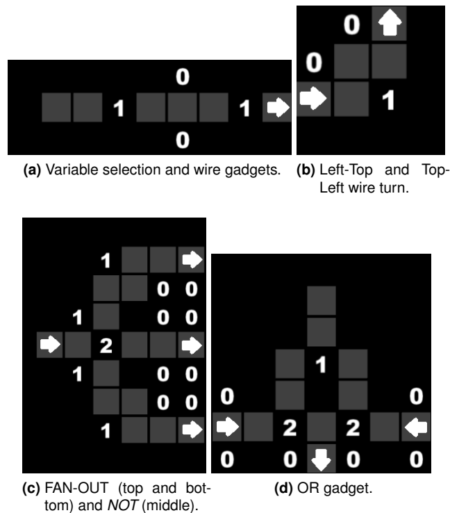
Figure 2.6: Akari's gadgets NP-Hard.
