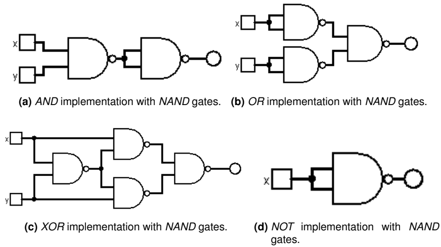
Figure 3.1: Individual gate conversion to NAND gates only.
