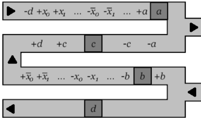
(c) TQBF universal quantifier gadget for x .
