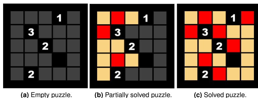
Figure 2.5: Puzzle example.
