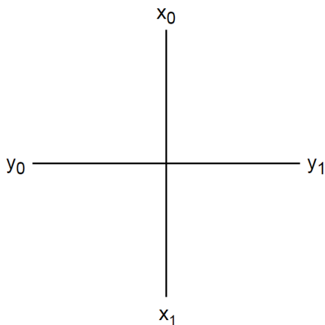
Figure 2.1: Crossover.
